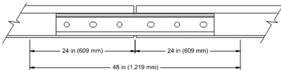
Figure 9-1 Location of Non-defective Tie at Joints - Class 1 and Class 2 tracks
