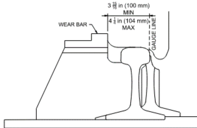
Figure 13-1 Limits for Adjustable Switch Point Guard
