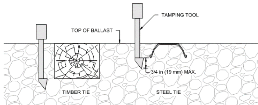
Figure 12-1 Tamping Head Depth Below Steel Tie
