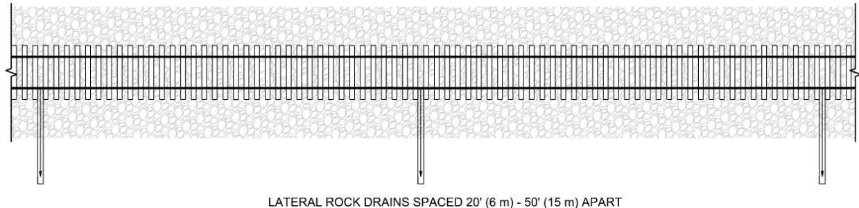
Figure 21-1 Lateral Rock Drains
