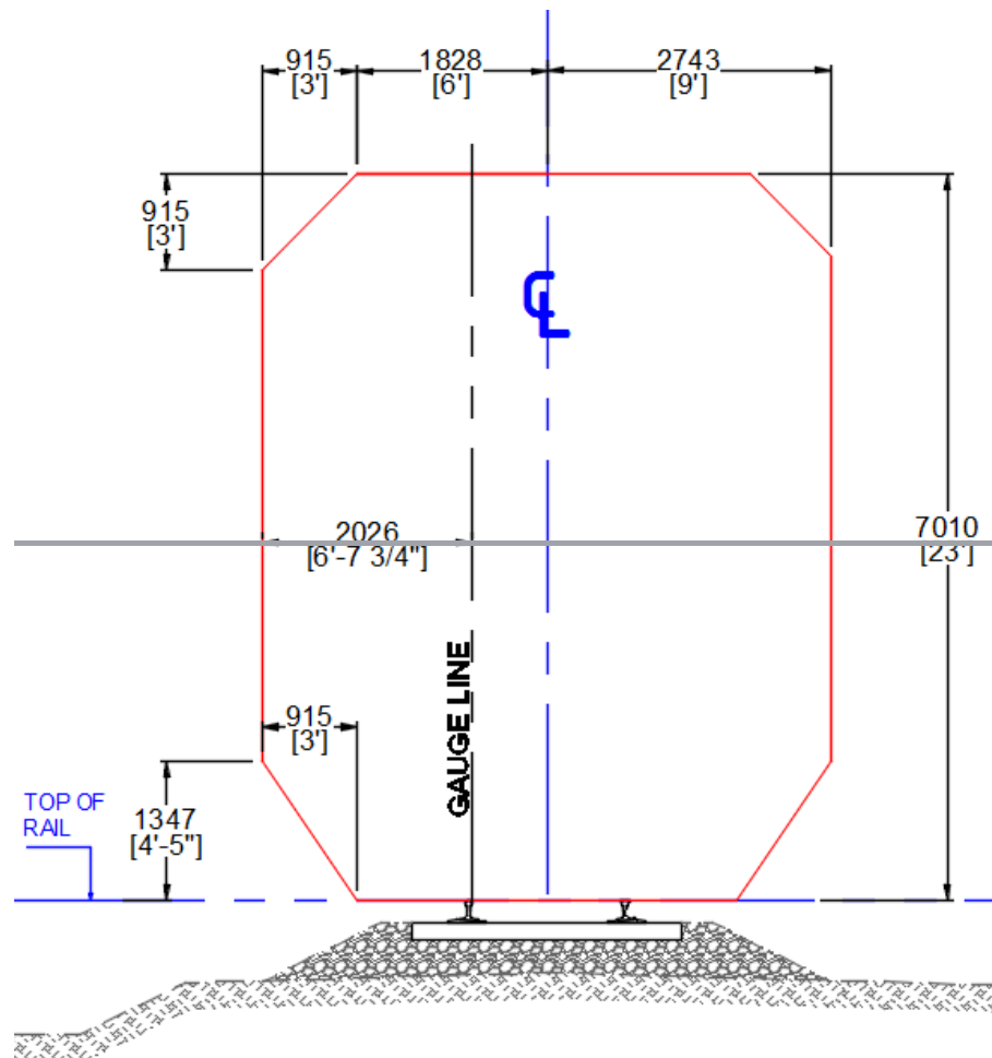
Figure X-2 Train Envelope for Bridges and Structures
