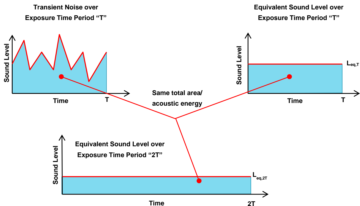
Figure 2-1: Equivalent Sound Level Concepts
