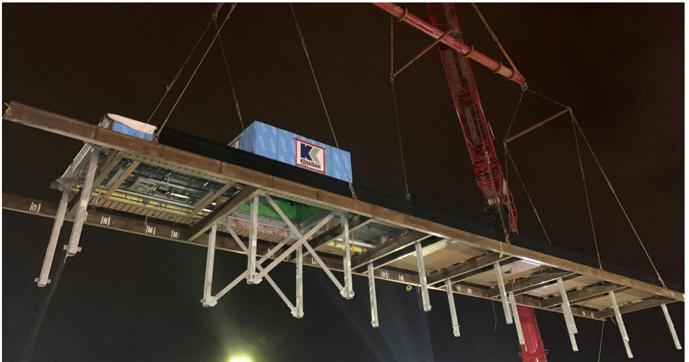
An image of the North Platform being hoisted into place by Kenaidan during the week of March 27.
