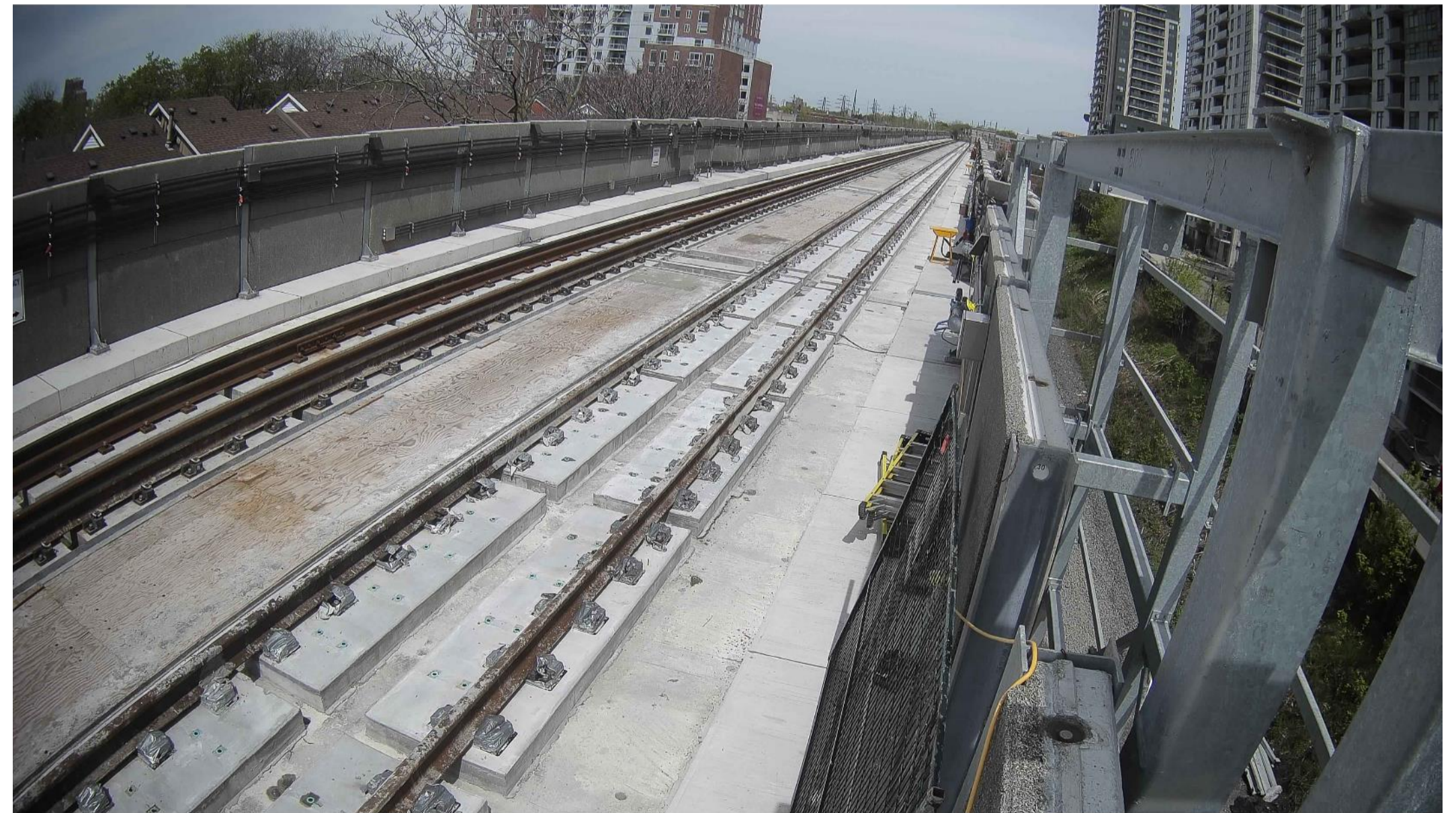
North facing view of the east and west mainline track near Antler St.
