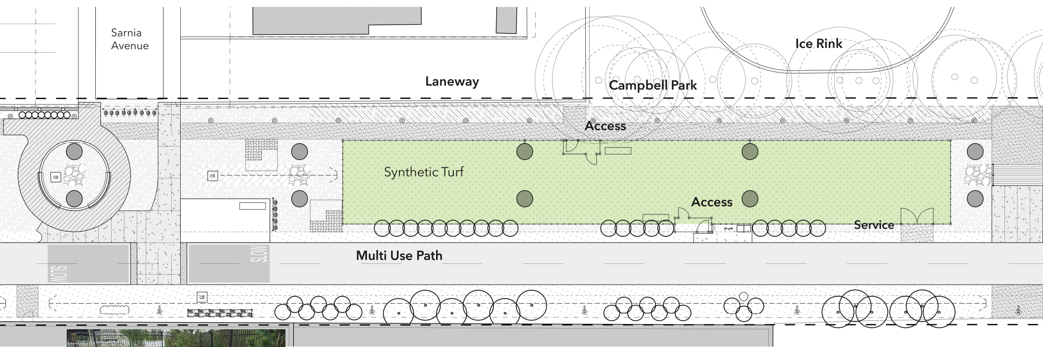
Synthetic Turf
