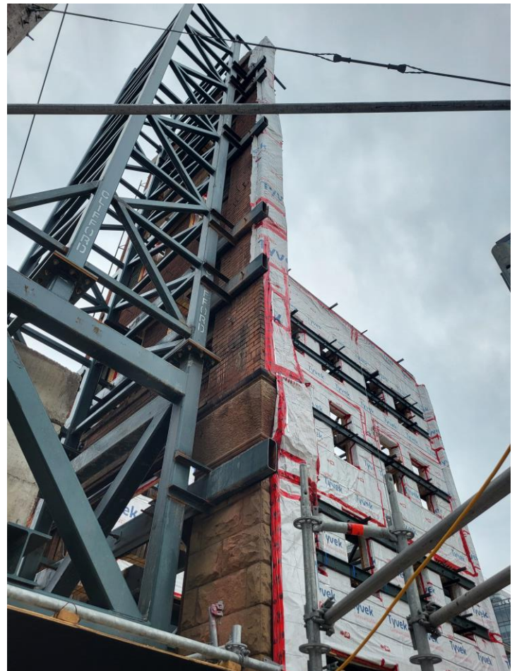
Retention tower installed in support of King-Bathurst heritage facade along King Street West.
