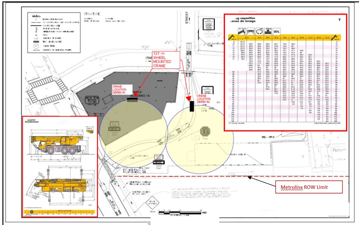
Figure A6: Sample Crane Swing Plan
