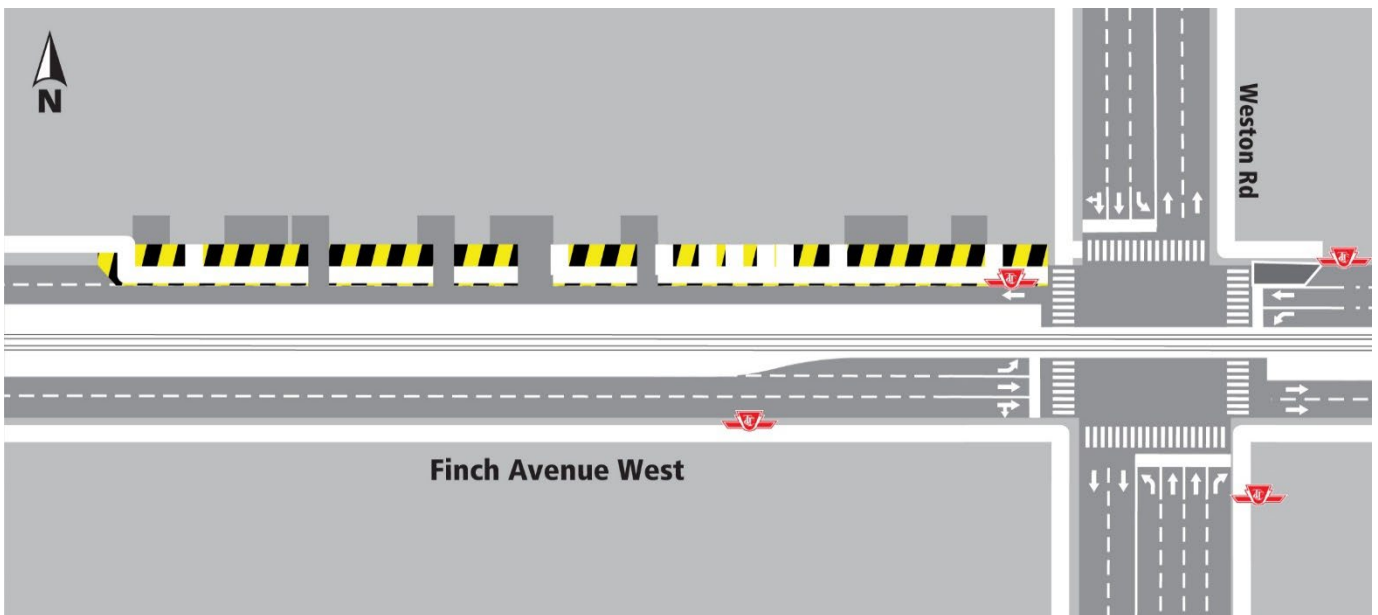
Map Description: Weston Road and Finch Avenue West. Temporary driveway closures will be implements as needed. Access to properties will remain at all times. Sidewalk works starting May 27, 2024, for three (3) weeks, approximately.
