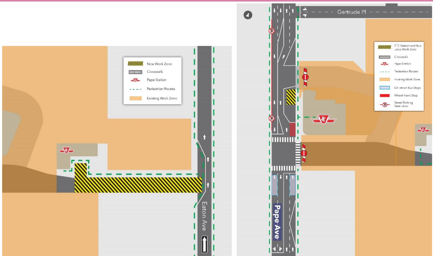
Work Zone 1 - Eaton Avenue
