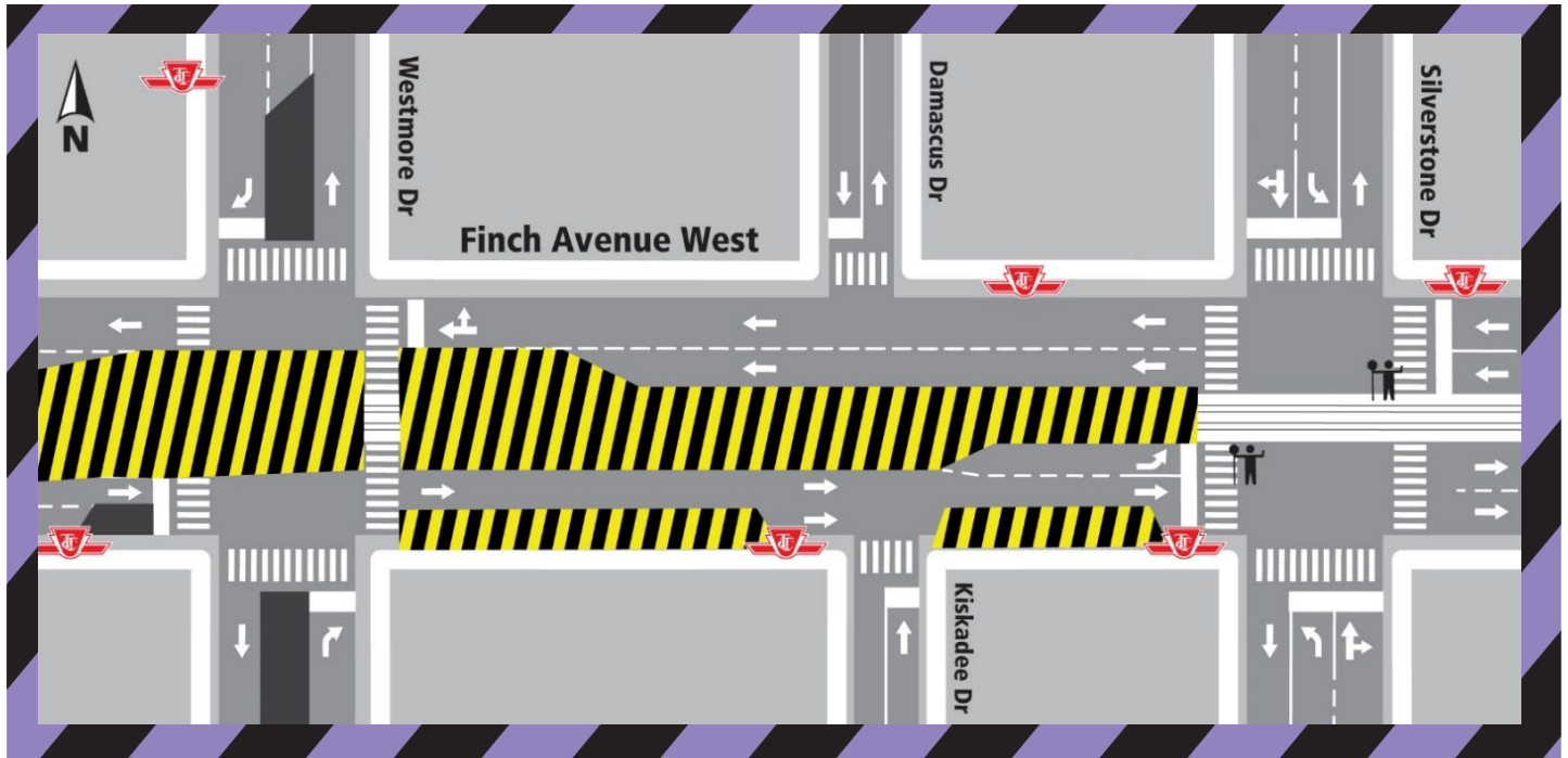
Map 1 Description: Westmore Drive to Silverstone Drive. Road and curb works. May 21, 2024 till June 17, 2024, approximately.
