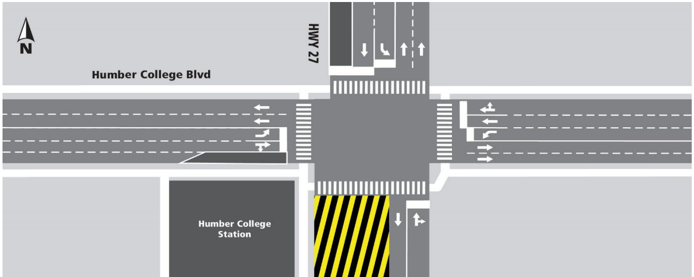
Map 2 Description: Humber College Boulevard to Hwy 27. Final paving starting June 19, 2024 for one (1) day, approximately.
