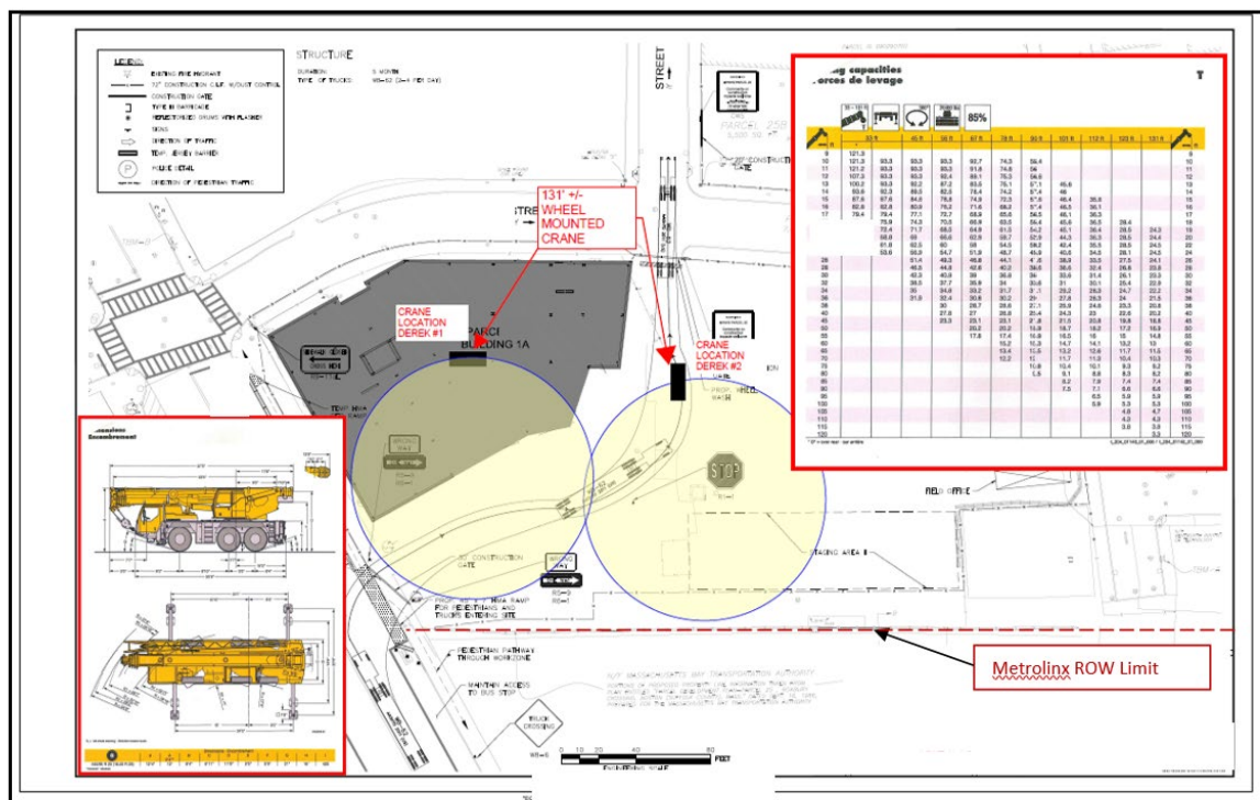
Figure A6: Sample Crane Swing Plan
