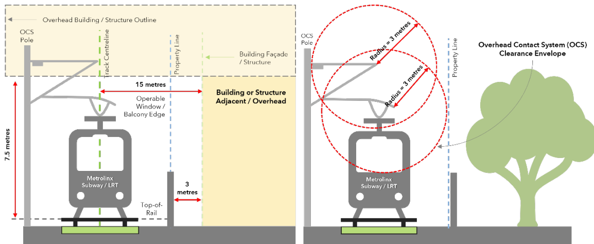
Figure A1: Adjacent Building or Structure Clearances
