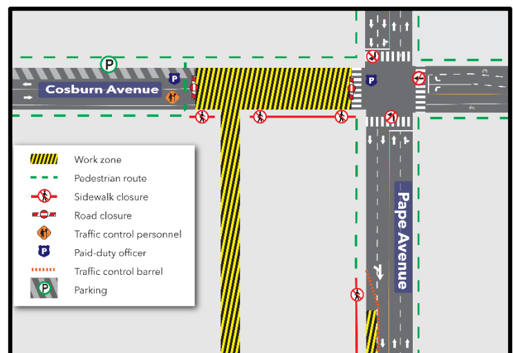
Figure 2: Full closure traffic staging
