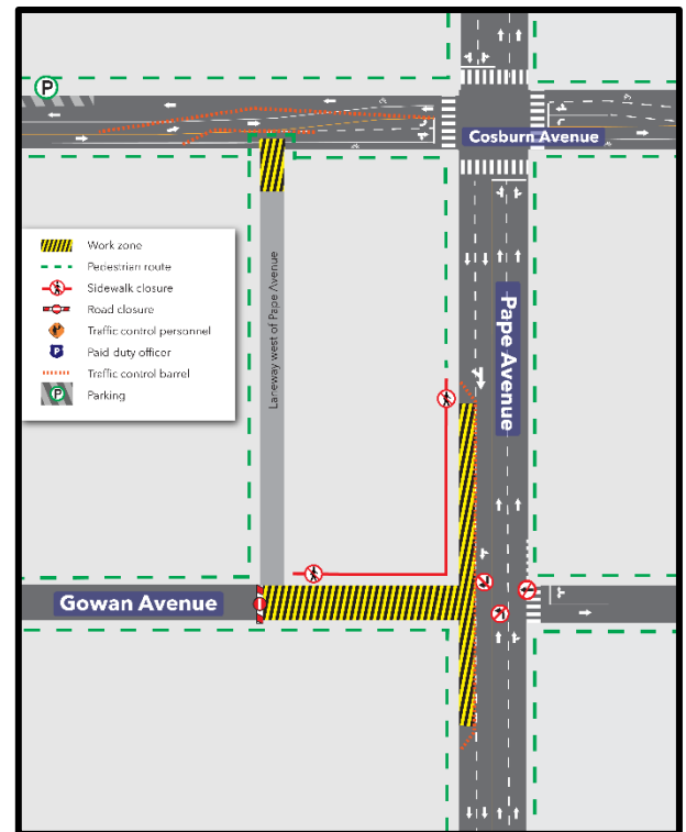
Figure 1: Bi-directional traffic staging
