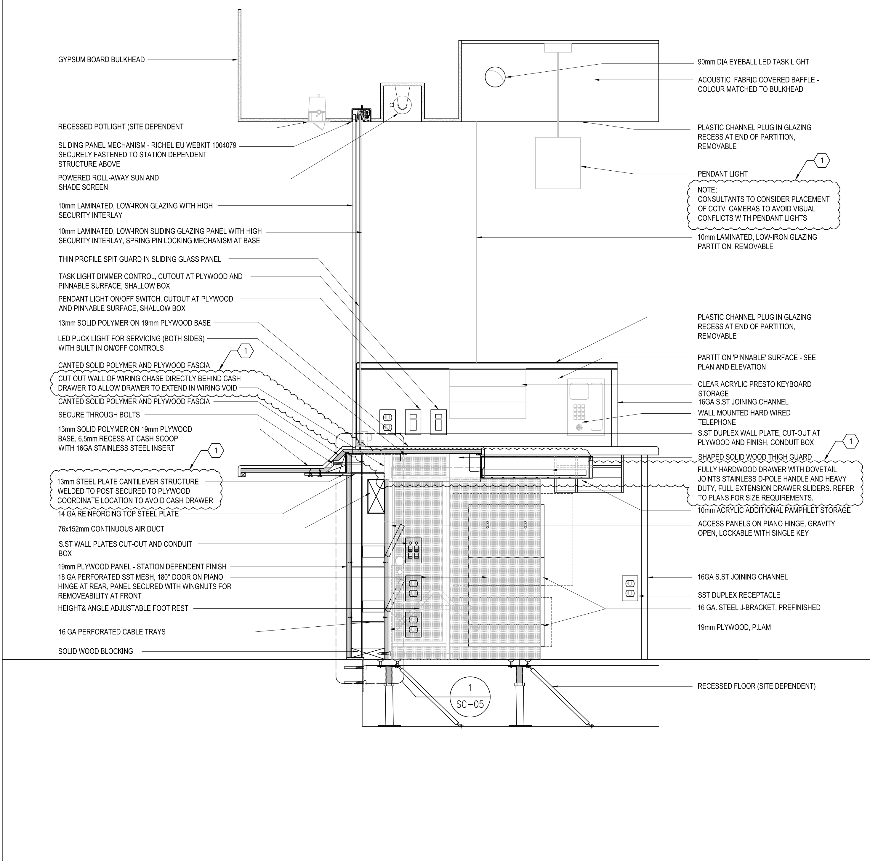
1 SECTION - THROUGH CASH DRAWER SCALE: 1:10
