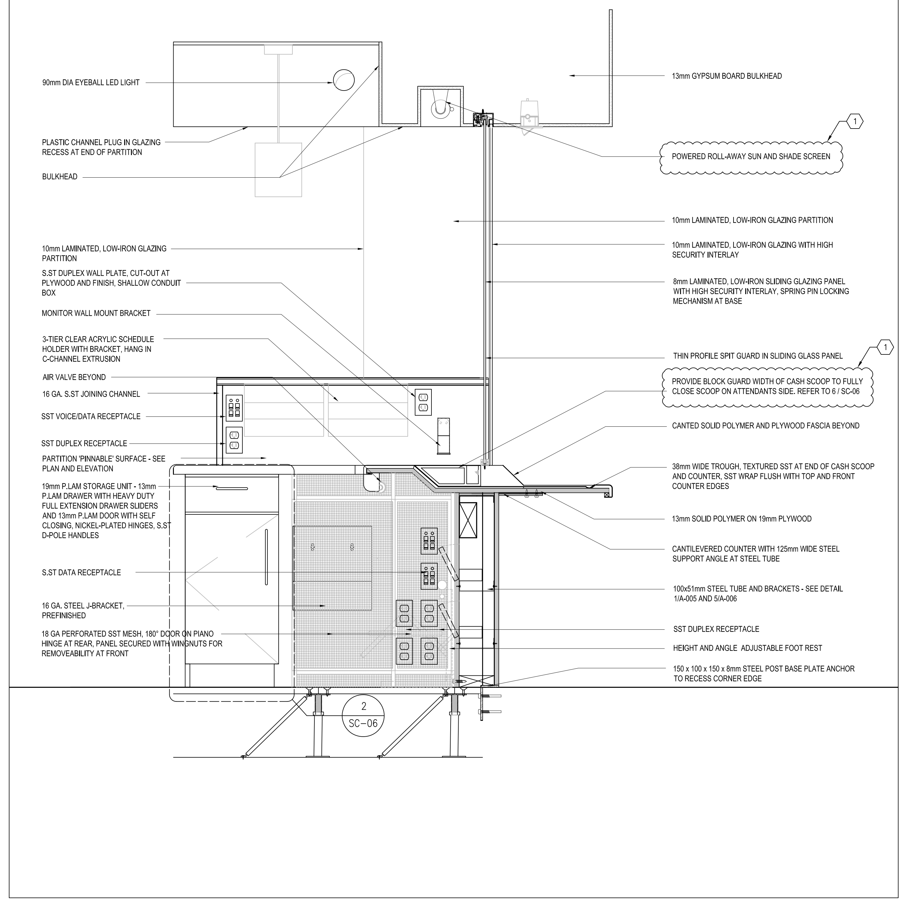
2 SECTION - THROUGH CASH SCOOP SCALE: 1:10
