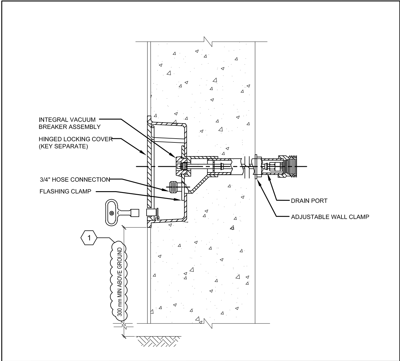
1 NON-FREEZE HOSE BIB DETAIL (WALL MOUNTED) M-100 SCALE : N.T.S.
