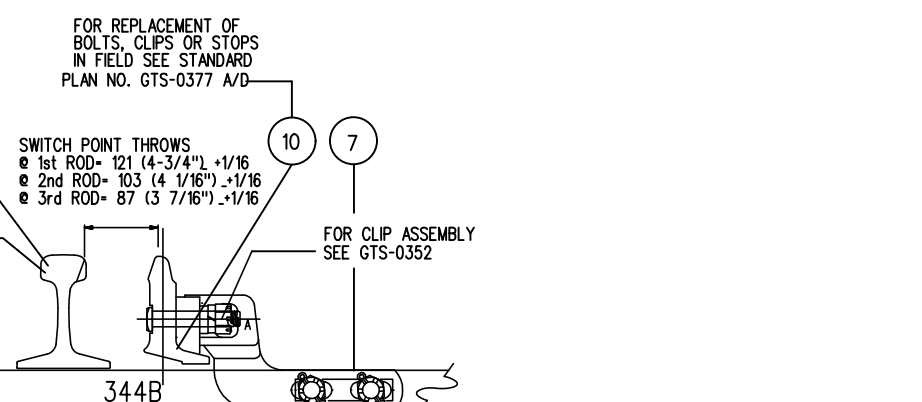
"MJS" CLIP ASSEMBLY
