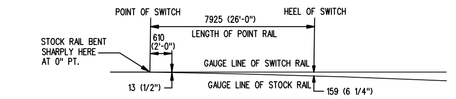
STOCK RAIL BENDING DETAIL
