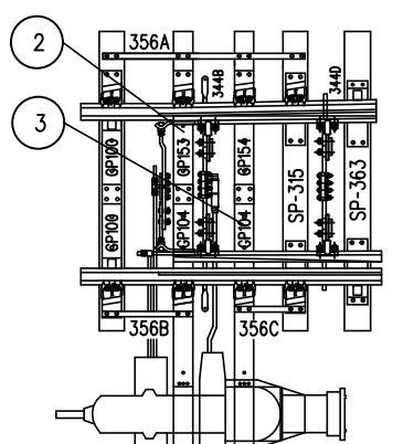
DRAWING NO. GTS-0251 C LEFT HAND TURNOUT MACHINE MOUNTED ON RIGHT
