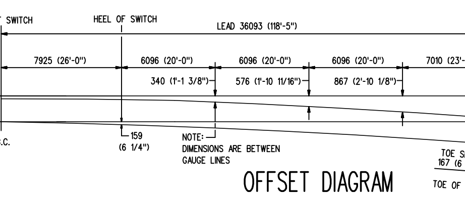
OFFSET DIAGRAM
