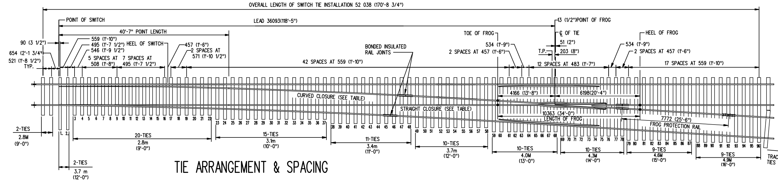
TIE ARRANGEMENT & SPACING
