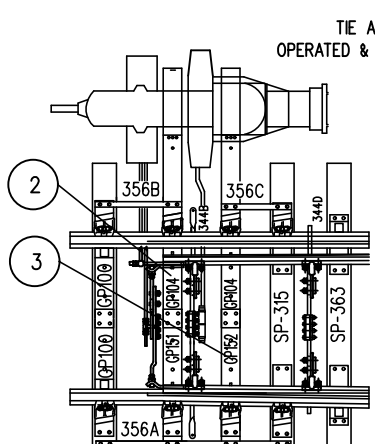
DRAWING NO. GTS-0251 B RIGHT HAND TURNOUT MACHINE MOUNTED ON LEFT
