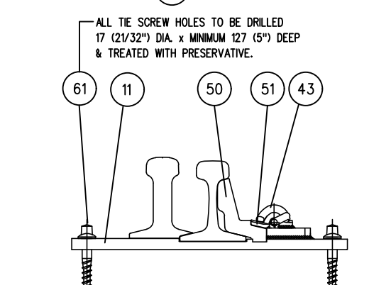
ADJUSTABLE RAIL BRACE ASSEMBLY
