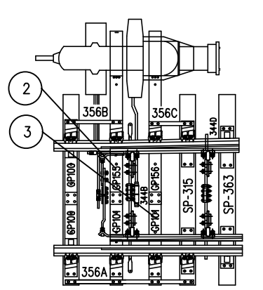
DRAWING NO. GTS-0251 D LEFT HAND TURNOUT MACHINE MOUNTED ON LEFT
