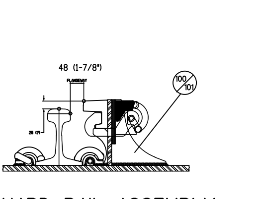
GUARD RAIL ASSEMBLY FOR REPLACEMENT STOCK NUMBERS OF WEAR BARS SEE GTS-1122
