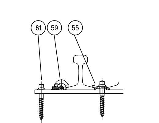
HOLD-DOWN CLIP ASSEMBLY
