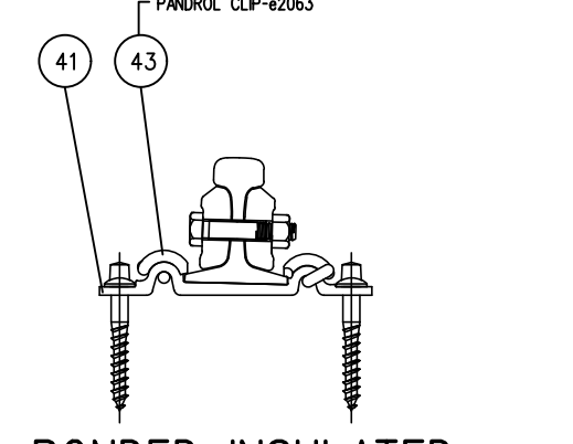
BONDED INSULATED RAIL JOINT
