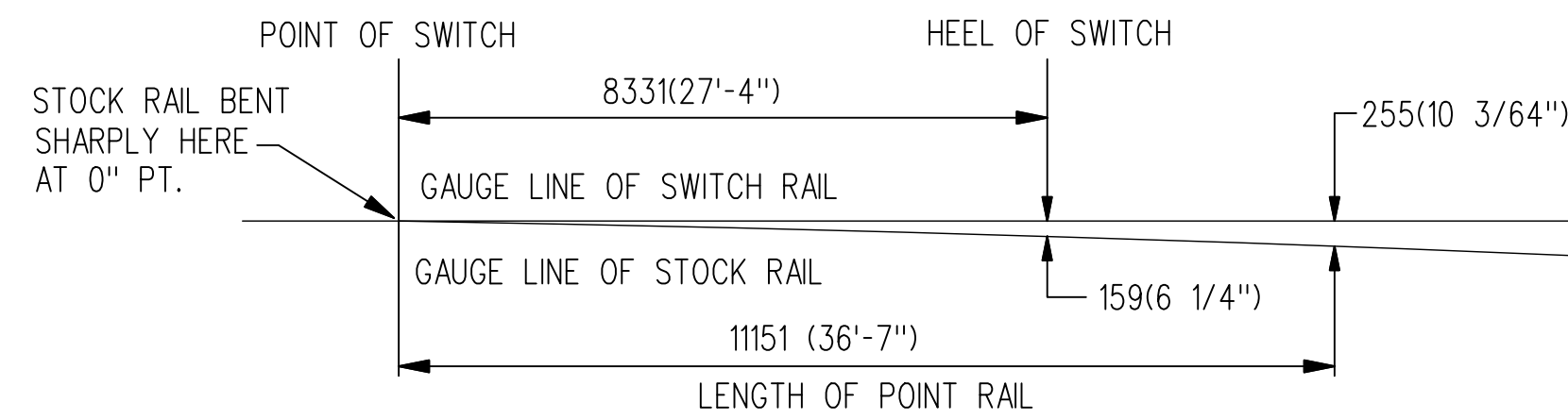
STOCK RAIL BENDING DETAIL
