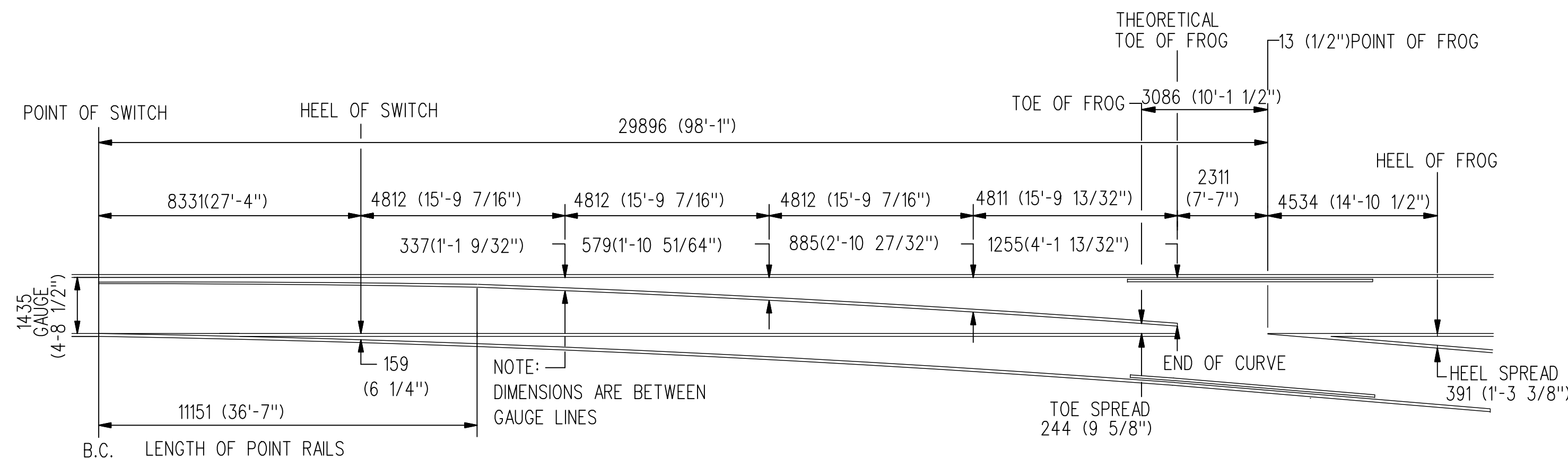
OFFSET DIAGRAM
