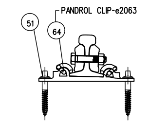
BONDED INSULATED RAIL JOINT
