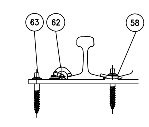
HOLD-DOWN CLIP ASSEMBLY
