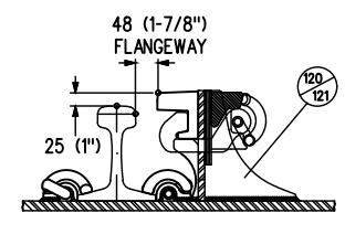
BOLTLESS GUARD RAIL ASSEMBLY
