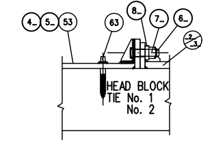
SWITCH MACHINE PLATE ASSEMBLY
