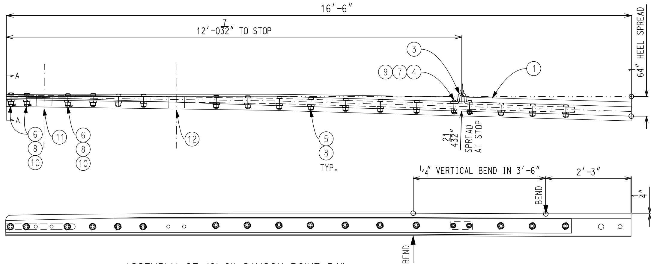
ASSEMBLY OF 16'-6" SAMSON POINT RAIL RIGHT HAND SAMSON POINT RAIL - GTS 320 A LEFT HAND SAMSON POINT RAIL - GTS 320 B (ILLUSTRATED)
