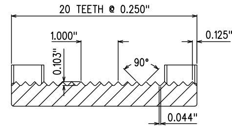
SERRATION DETAIL
