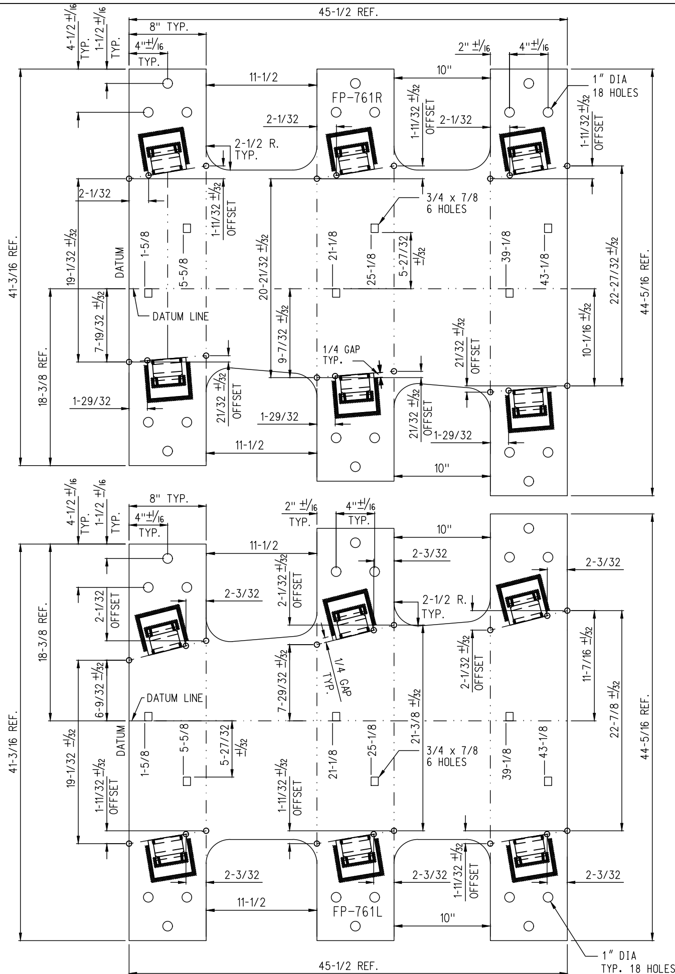
FROG BASE PLATE FP761L WEIGHT 341LBS. REPLACES FP-442L
