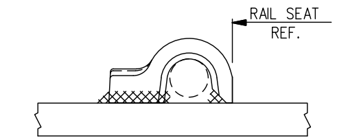
PANDROL SHOULDER DETAIL
