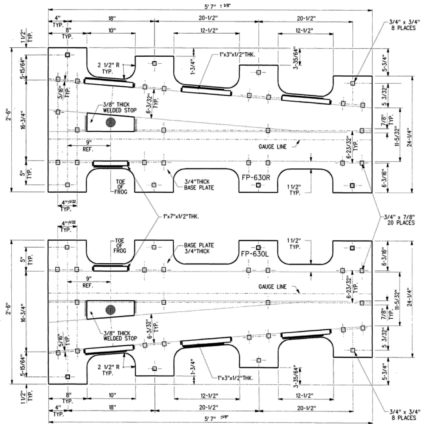
FROG BASE PLATE FP-630R
