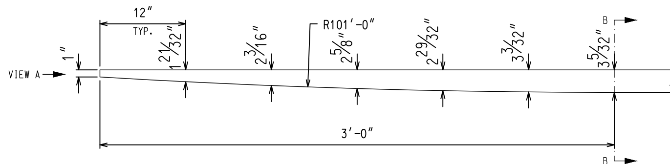
FLARE MACHINING DETAIL
