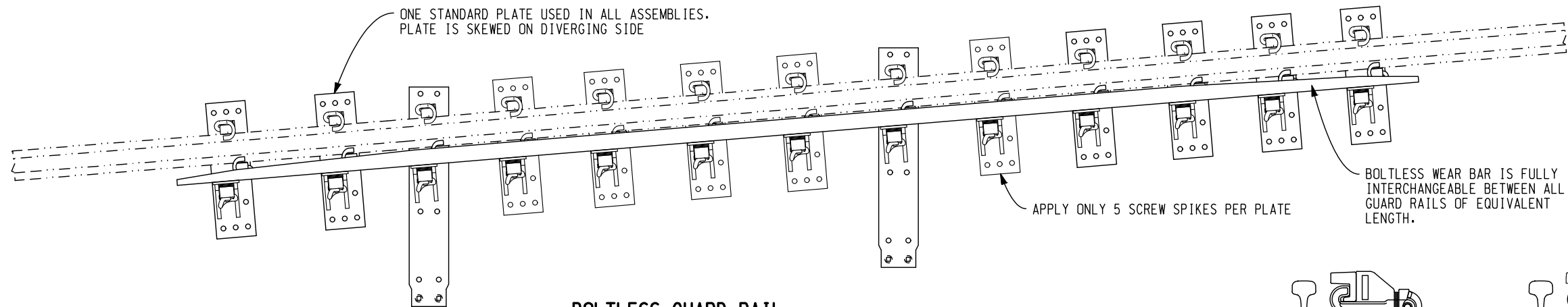
BOLTLESS GUARD RAIL (LEFT HAND ASSEMBLY - LEFT HAND TURNOUT SHOWN)
