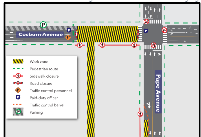
Figure 2: Full closure traffic staging
