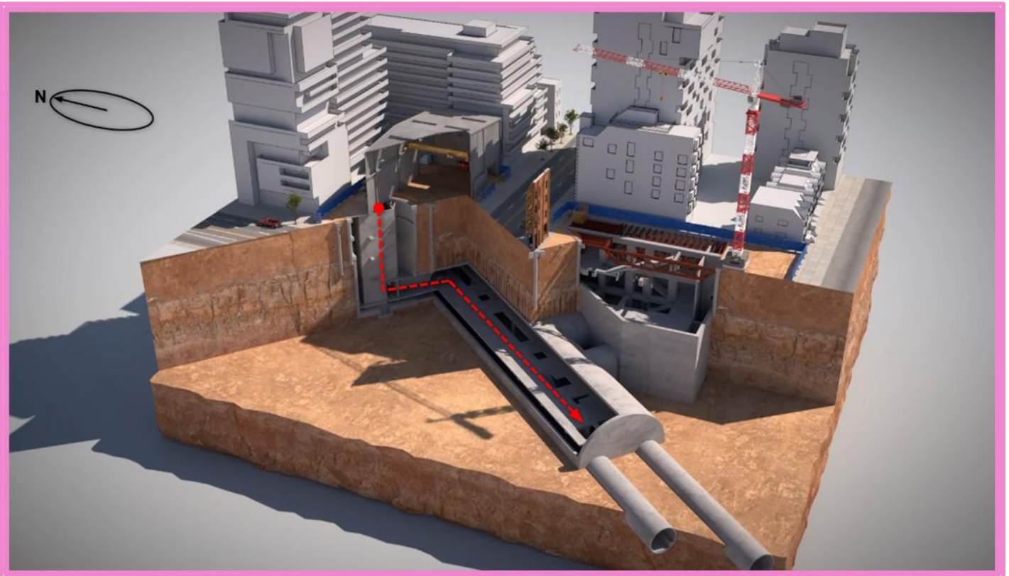
Diagram of the King-Bathurst cavern location and excavation direction.
