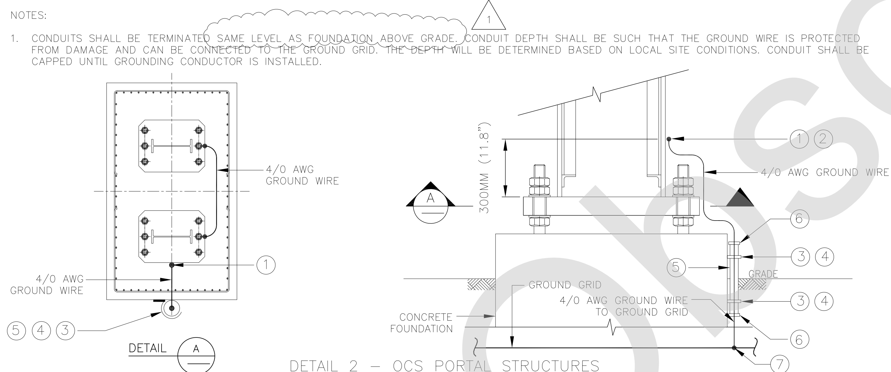
DETAIL 2 – OCS PORTAL STRUCTURES
