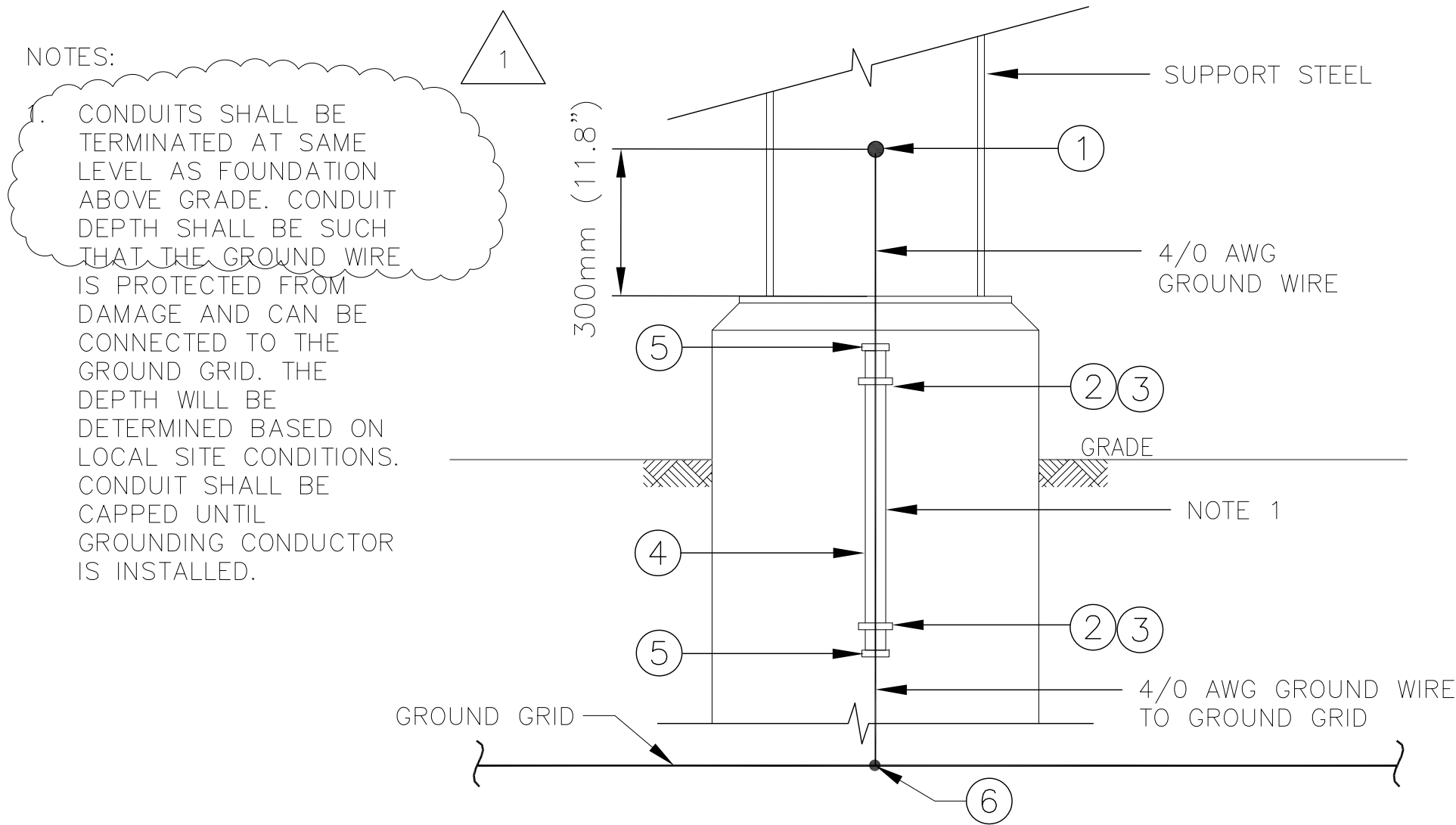
DETAIL 1 – LIGHTING POLES
