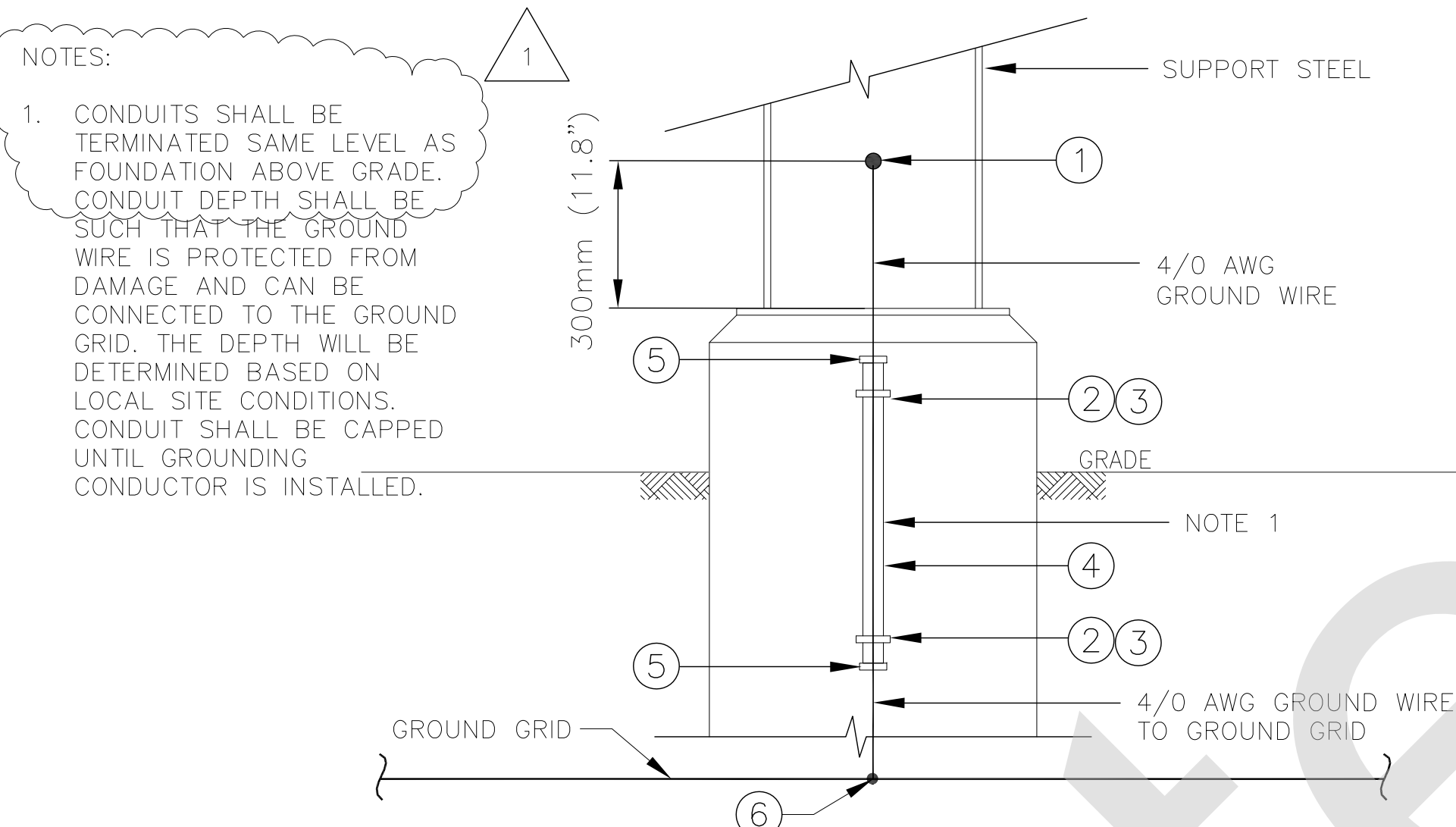
DETAIL 4 – PROTECTIVE CANOPIES AND CANOPY COLUMNS
