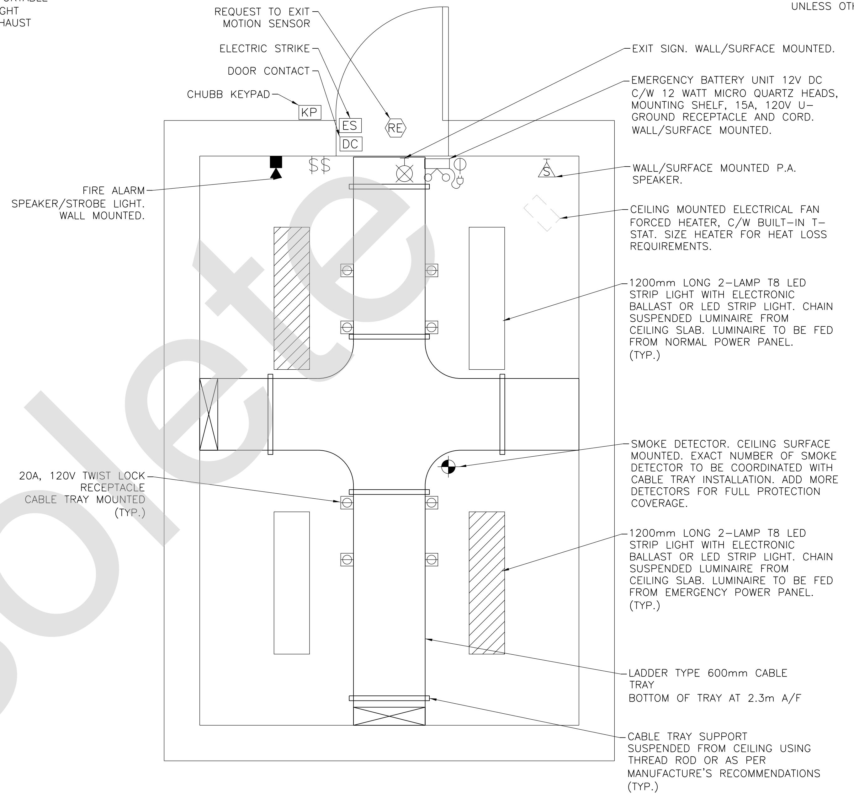
CEILING PLAN & FIRE ALARM PA PLAN
