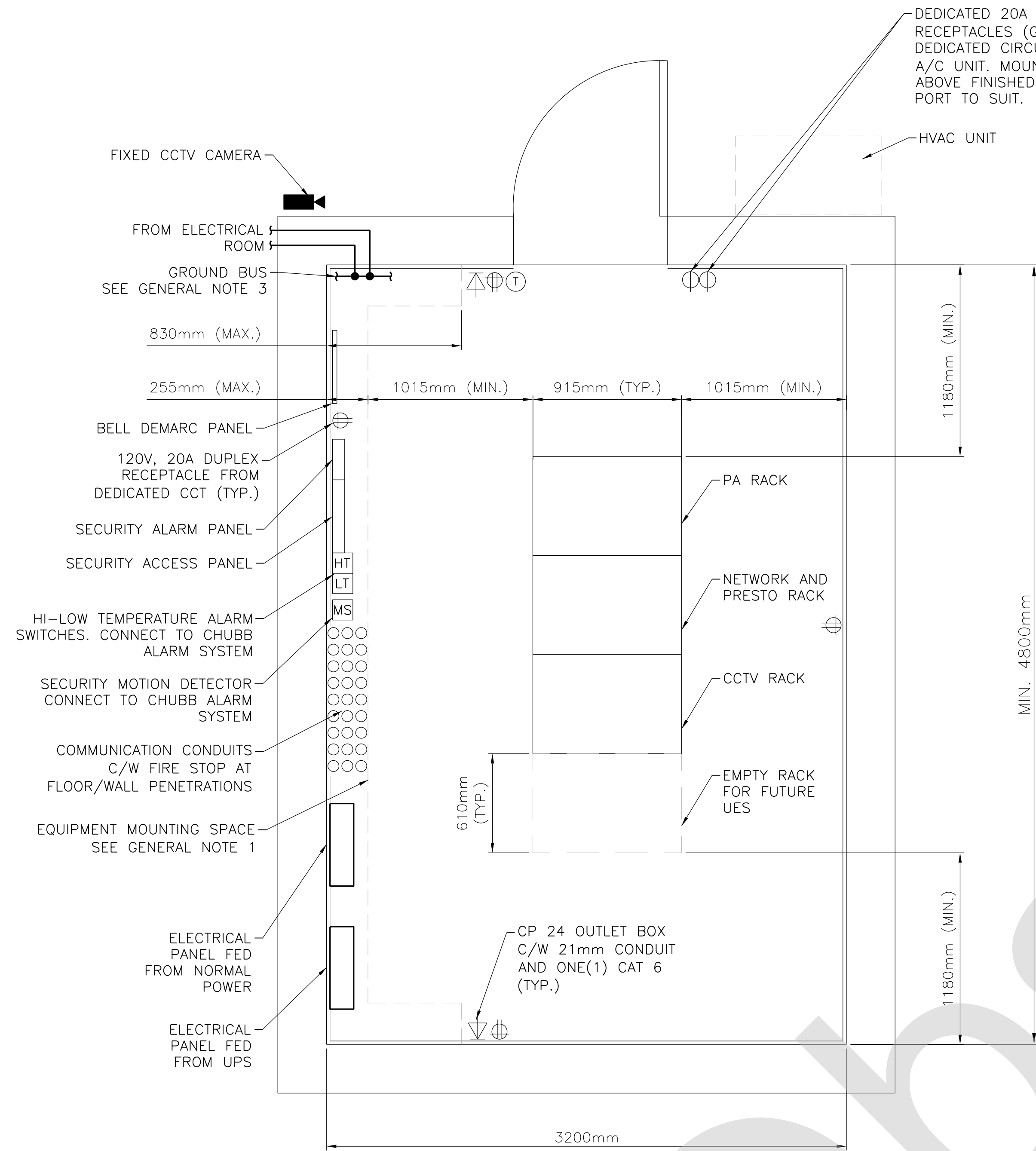
FLOOR PLAN
