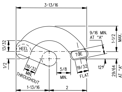
PANDROL RAIL CLIP TYPE e2009 FLAT TOE FOR CONCRETE TIES
