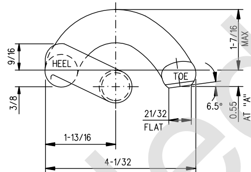
PANDROL RAIL CLIP TYPE e2055 FLAT TOE FOR WOOD TIES
