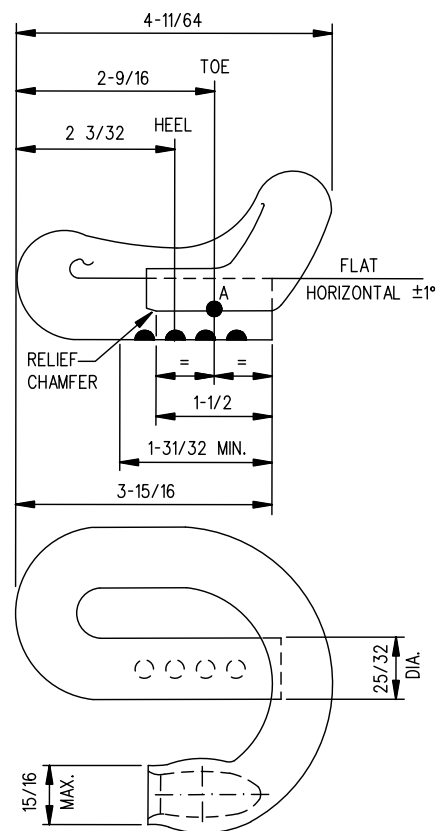
PANDROL RAIL CLIP TYPE e2009 FLAT TOE FOR CONCRETE TIES
