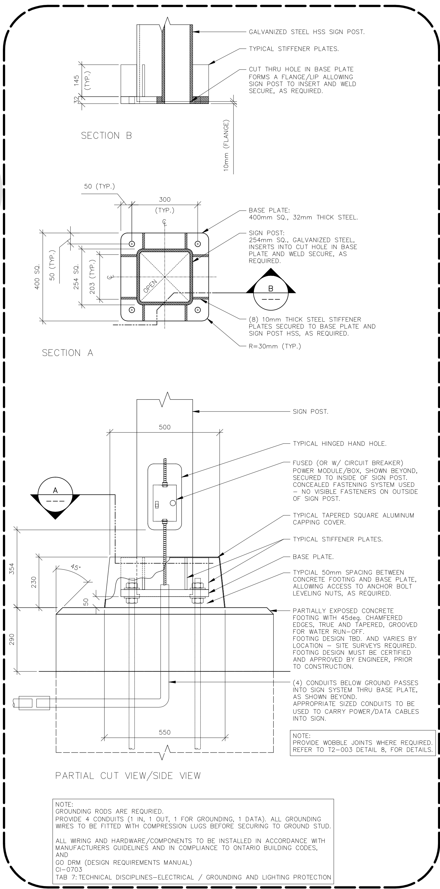
3 BASE PLATE DETAILS/SECTIONS Scale: 1:10
