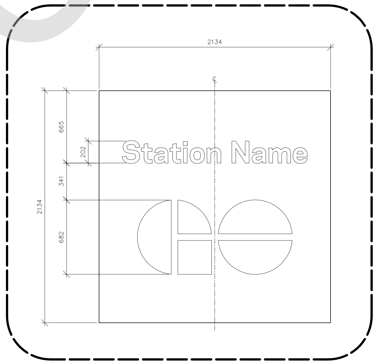
2B STATION NAME/LOGO DETAIL (1-LINE) Scale: 1:20
