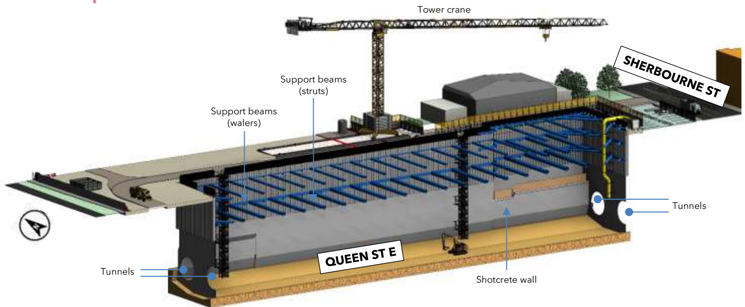
Diagram of the future advanced Moss Park station excavation.
