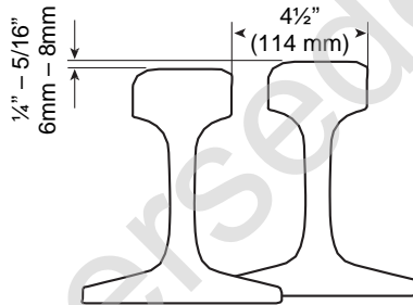
Figure 32. - Switch Point and Stock Rail Minimum Clearance
