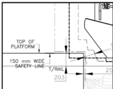
DETAIL 2 1:20
