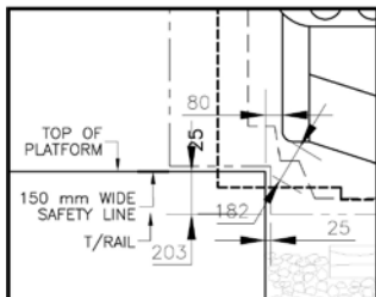
DETAIL 1 1:20
