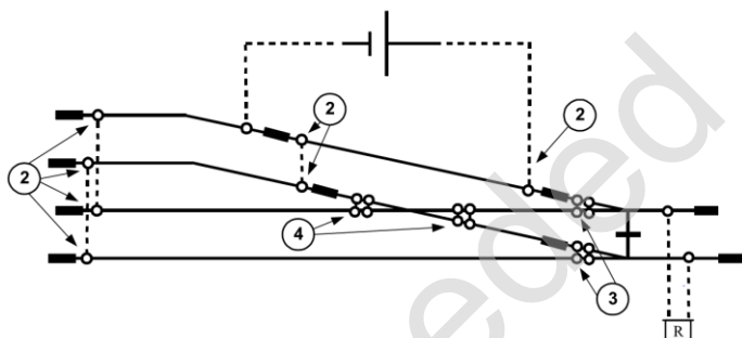
Figure 011-4: Series Fouling
