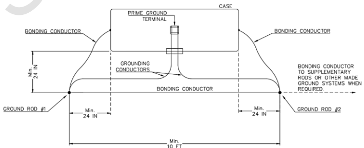
Figure 1102-6: Typical Grounding Arrangement at Cases
