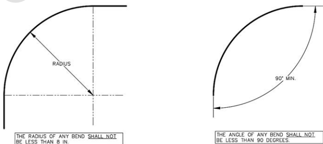
Figure 1102-3: Bending Conductors
