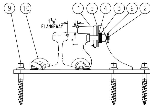
TYPICAL SECTION
