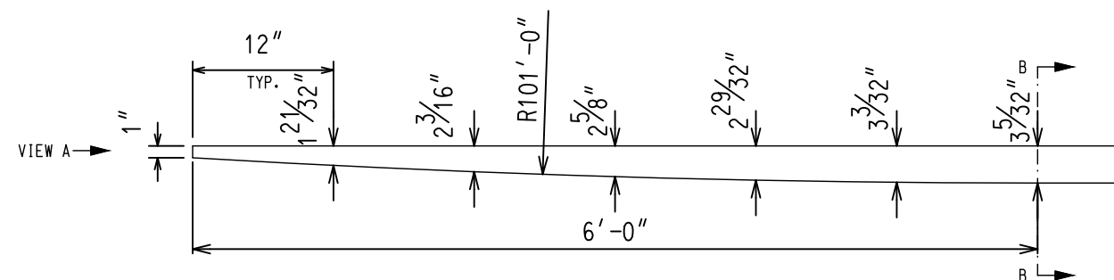
FLARE MACHINING DETAIL
