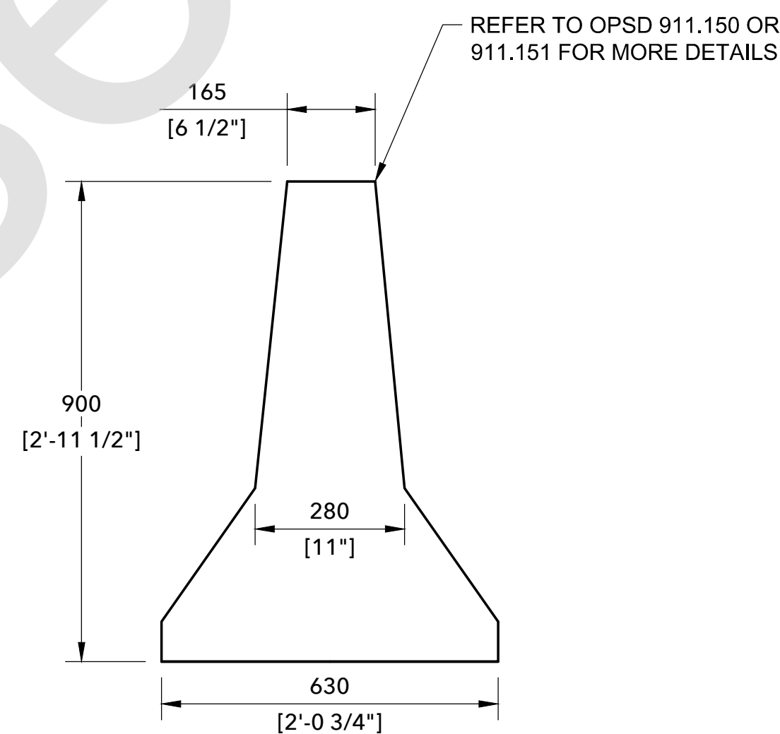
TEMPORARY CONCRETE BARRIER (TCB) ELEVATION
