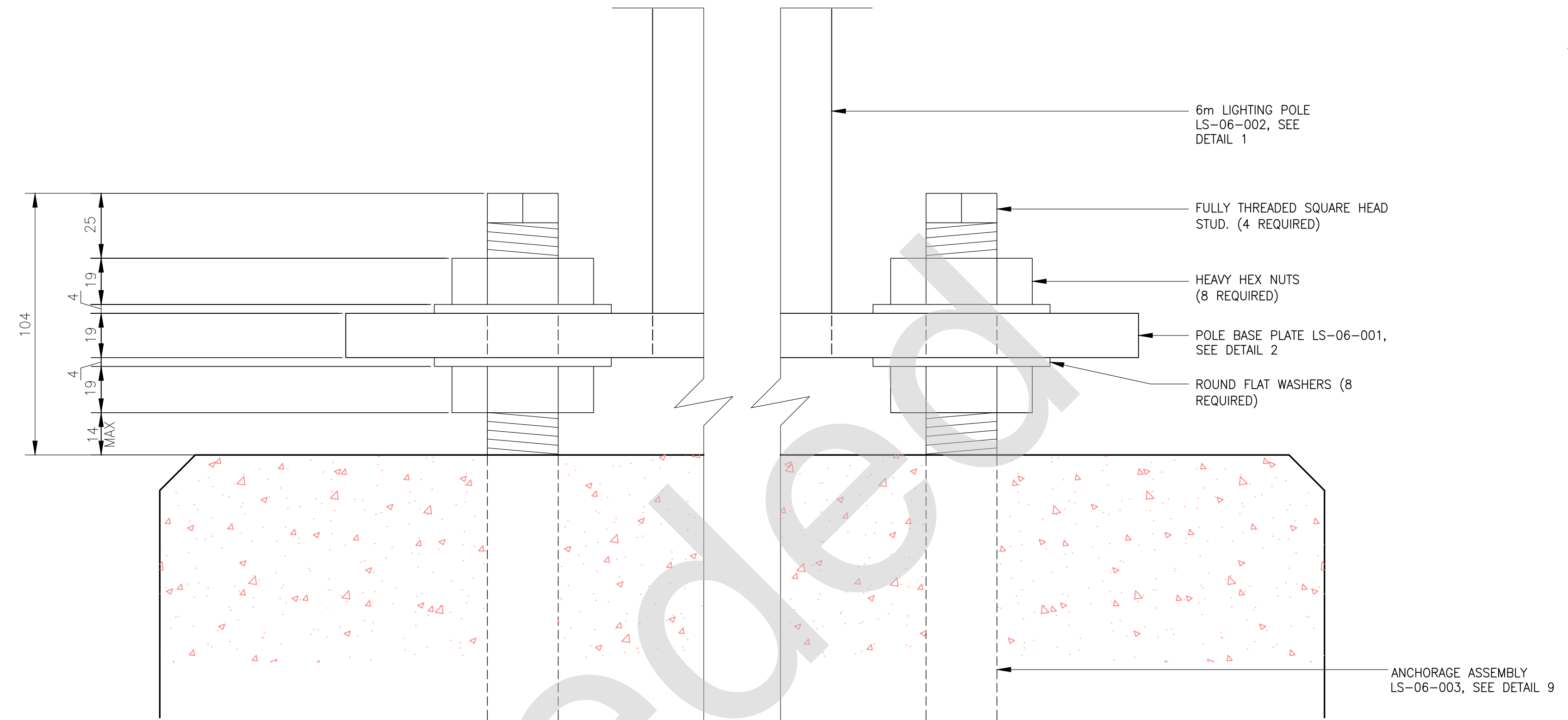
DETAIL 14 BASE MOUNTING LS-06-001, LS-06-002, LS-06-004
