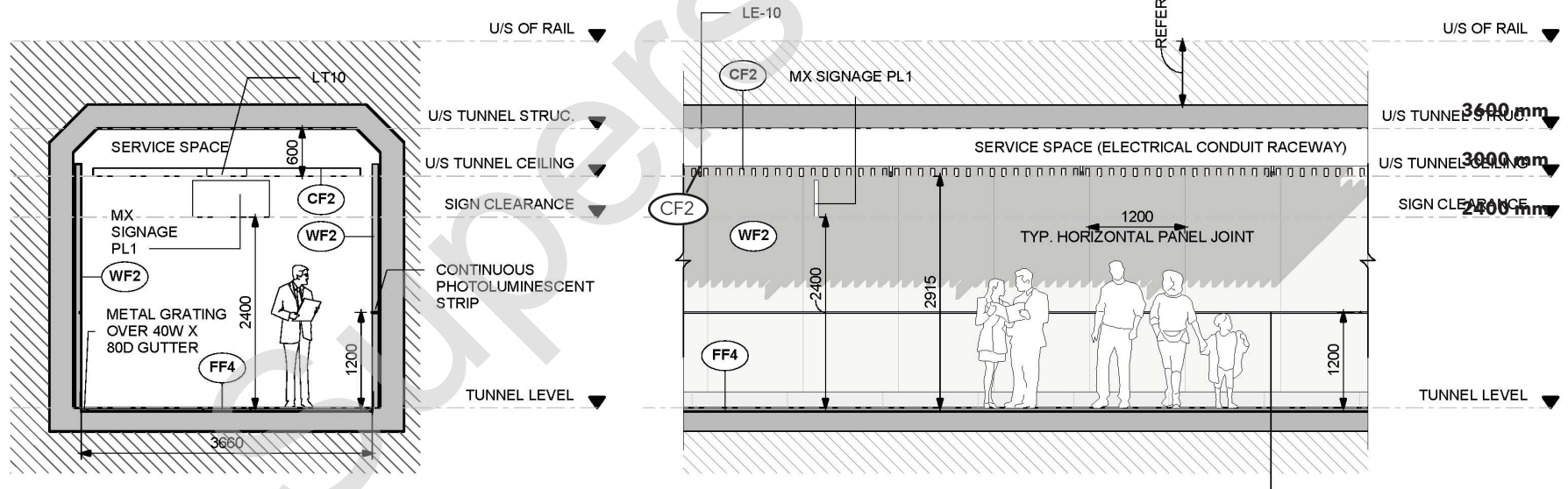
Figure 26: Illustration of tunnel showing ceiling raceway and wall finish
