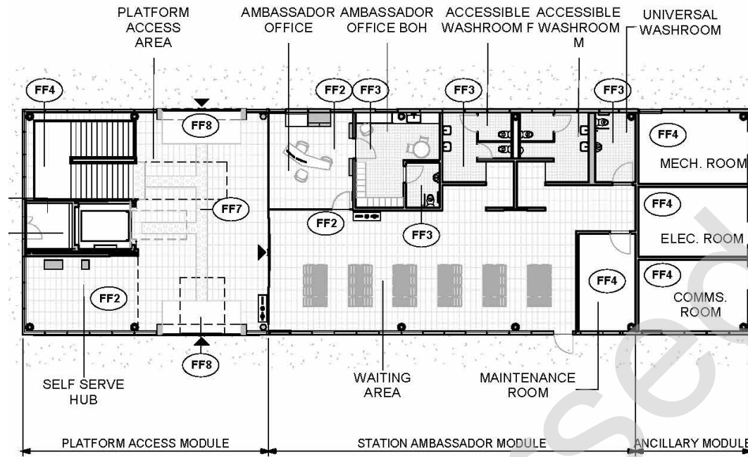
Figure 56: Interior Finishes Plan
