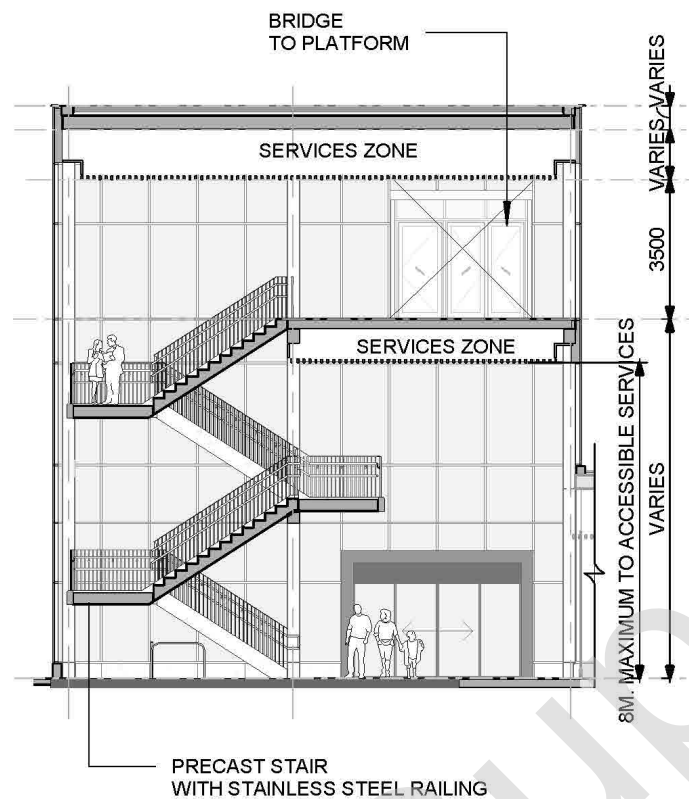
Figure12: Cross Section of Platform Access Module (Bridge configuration)
