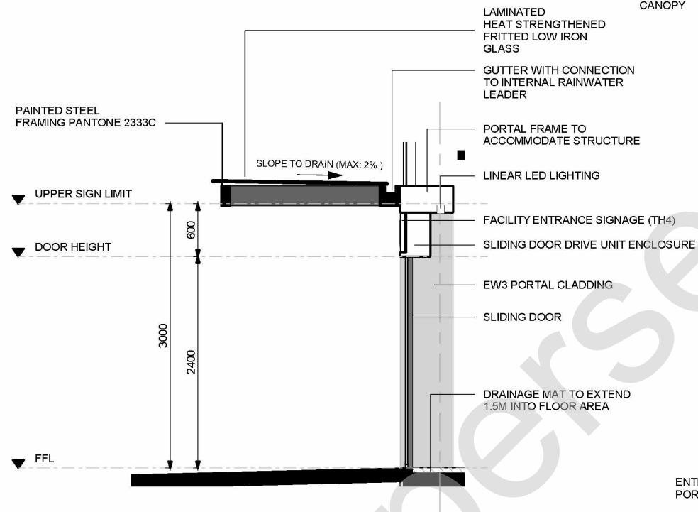
Figure 52: Section through entrance canopy. NOTE: Rain water leader from canopy to be housed within portal frame. Provide access panels in portal frame for clean-out.
