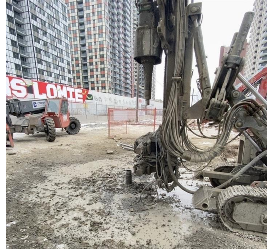
#5 Hydraulic drill rig used within rail corridor
