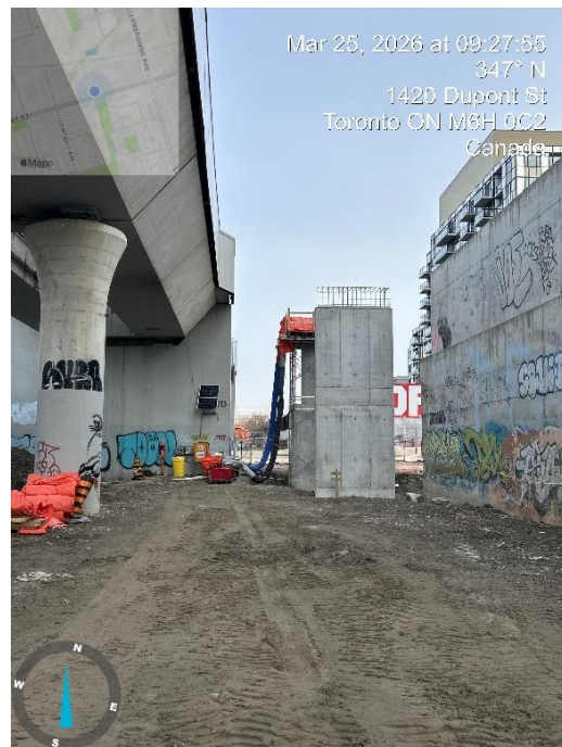
#4 South abutment of new pedestrian bridge
