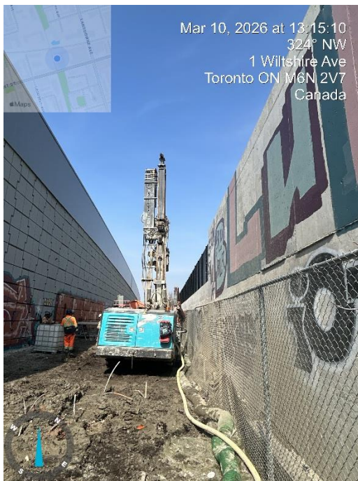
#1 Micropiling work for new pedestrian walkway
