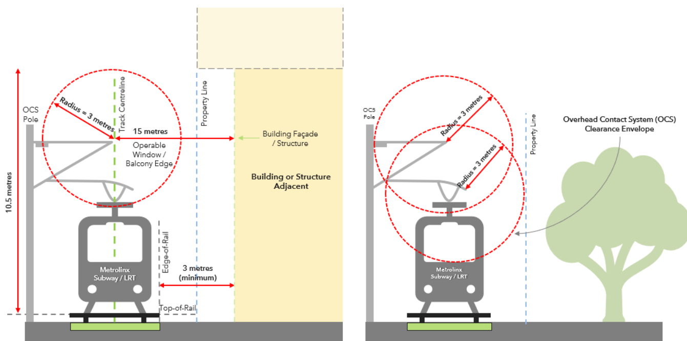
Figure A1: Adjacent Building or Structure Clearances
