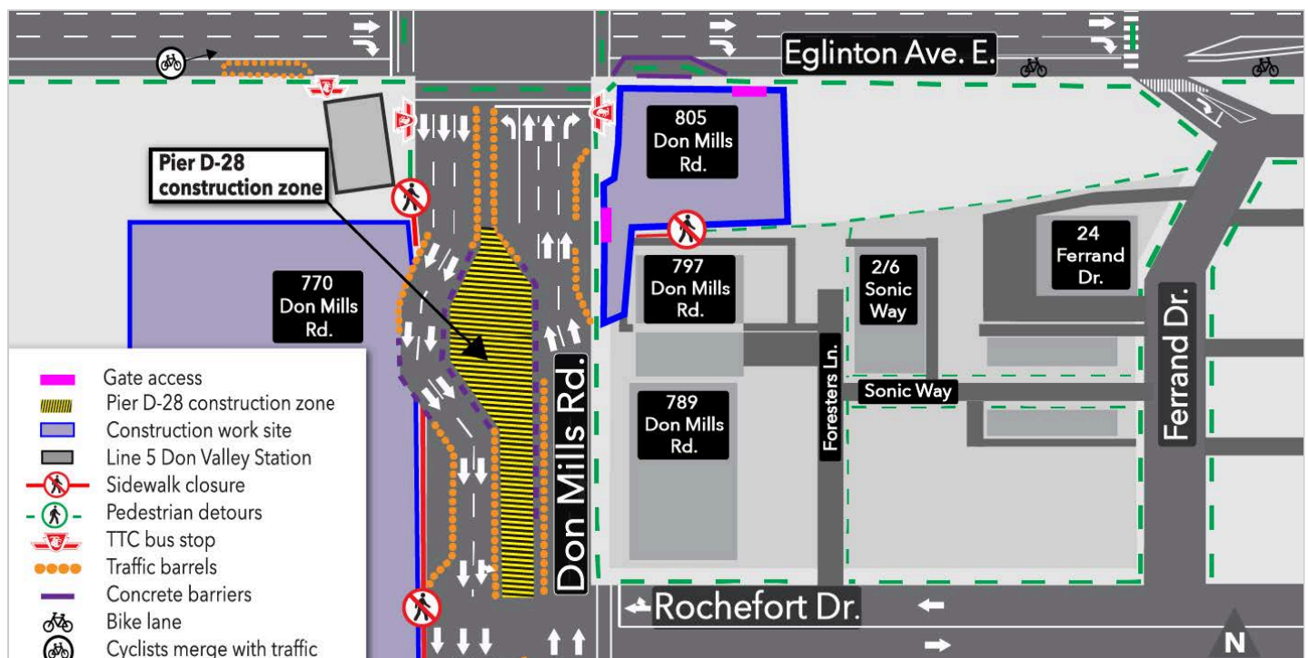
Map of Pier construction work for Pier D-28 at Don Mills Road between Eglinton Avenue East and Rochefort Drive
